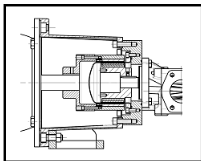
Abb. 7: Magnetkupplung
