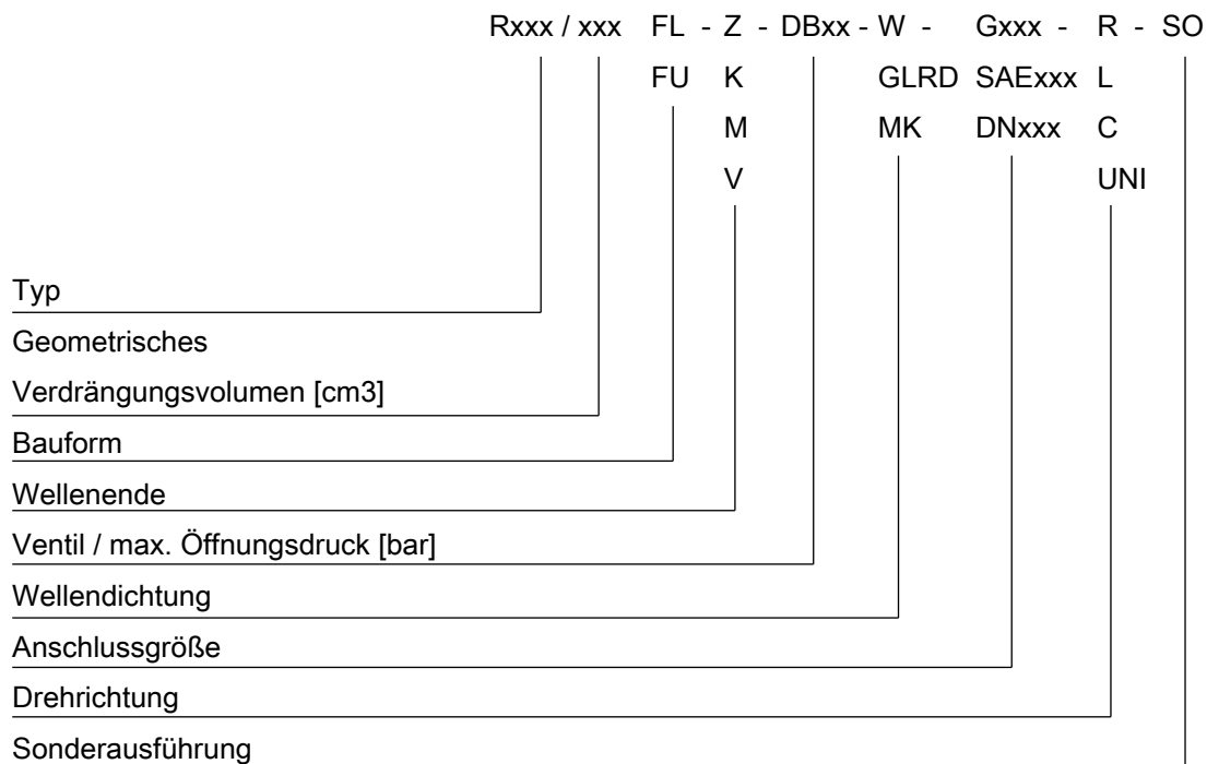
Abb. 8: Typenschlüssel
